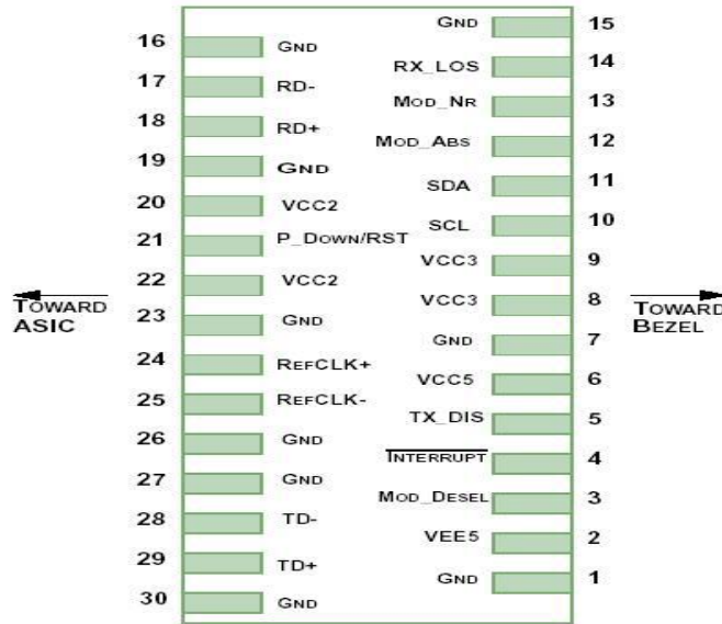
Figure1.Electrical Pin-out Details
